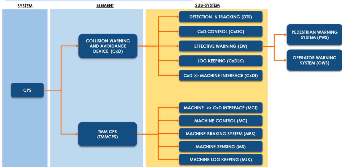
Figure 3: CPS functional breakdown structure
